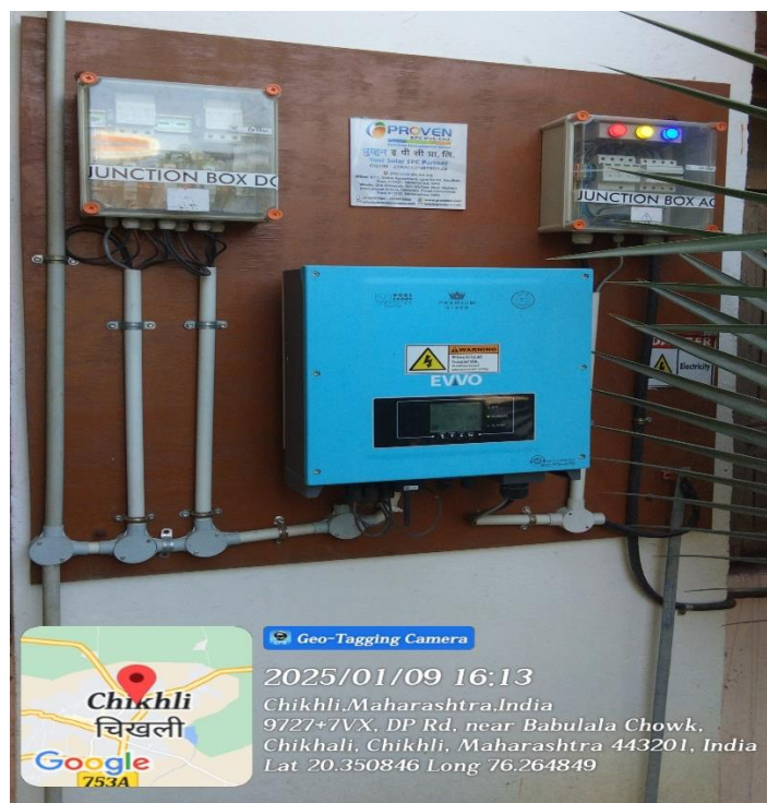
Solar Energy: Wheeling to the Grid
